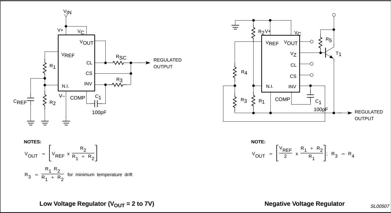
Figure 5. Typical Applications
