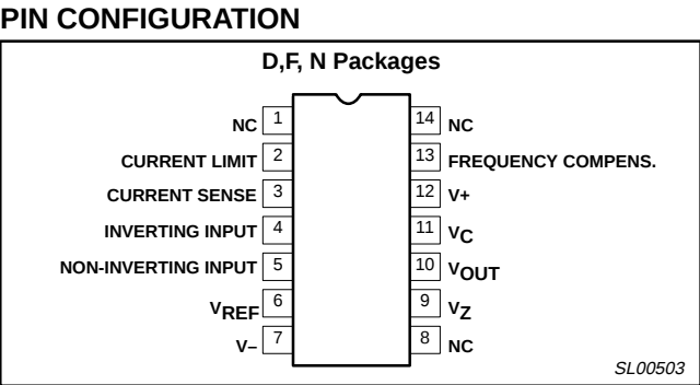
Figure 1. Pin Configuration
