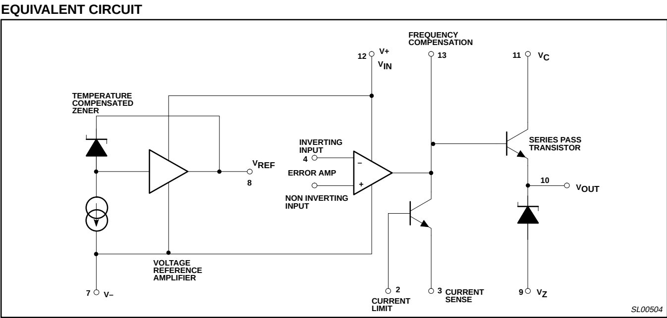
Figure 2. Equivalent Circuit
