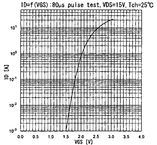
伝達特性 Typical transfer characteristics
