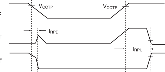
Figure 1. Power-Up/Power-Down Sequence
