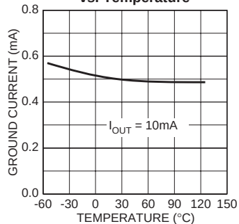
MIC2951x Ground Current vs. Temperature
