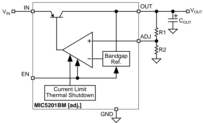
Adjustable Regulator
