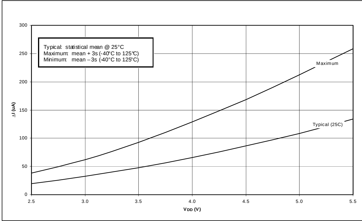
FIGURE 21-14: TYPICAL AND MAXIMUM \Delta I_{RPU} vs. V_{DD} (MEASURED PER INPUT PIN, -40°C TO +125°C)
