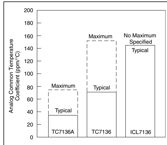
FIGURE 7-3: ANALOG COMMON TEMPERATURE COEFFICIENT
