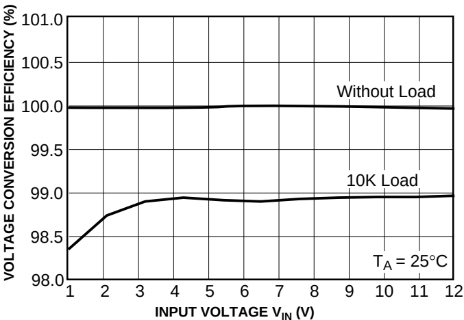
Voltage Conversion
