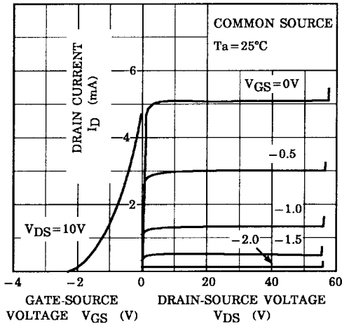
STATIC CHARACTERISTIC
