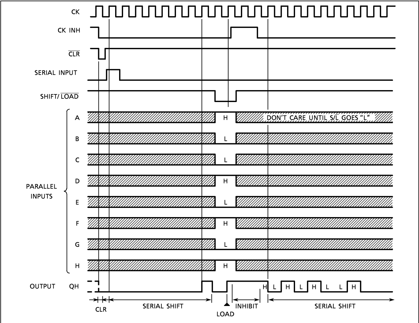
TIMING CHART
