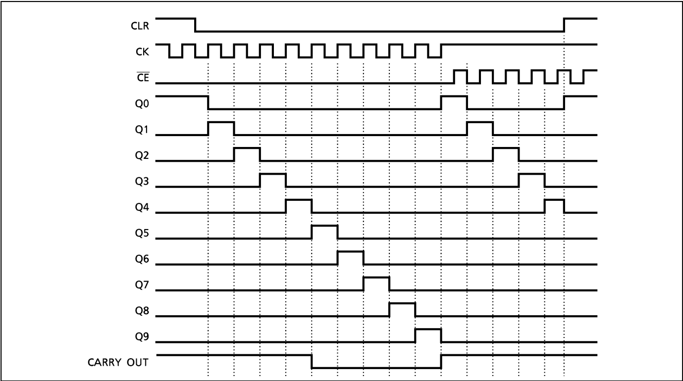
TIMING CHART
