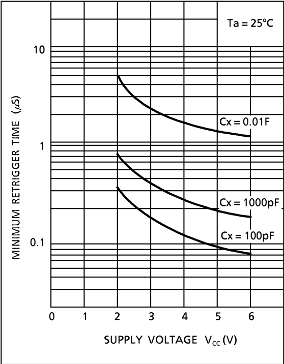
t_{rr} - V_{CC} CHARACTERSTICS ( TYP. )
