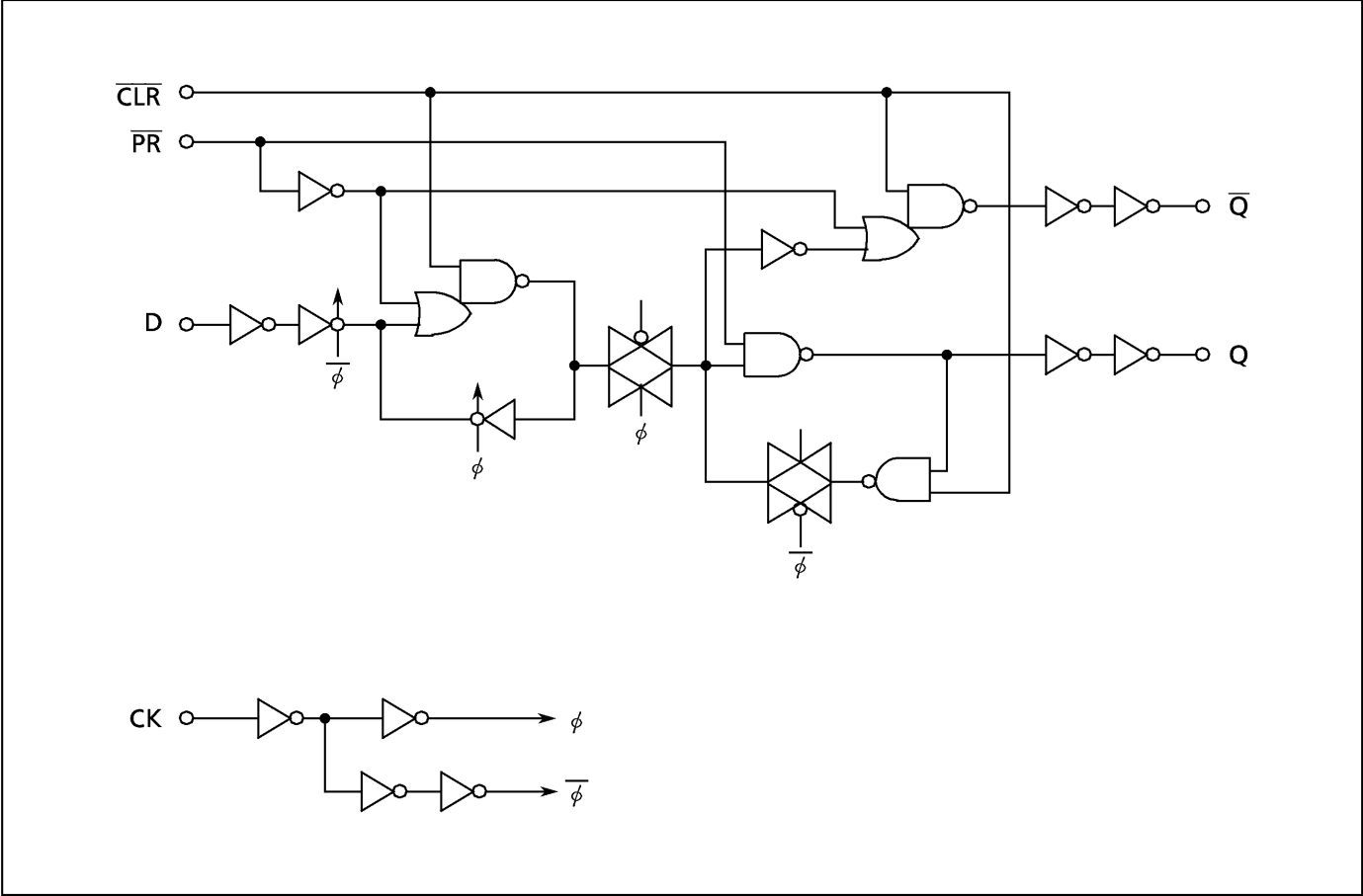
SYSTEM DIAGRAM
