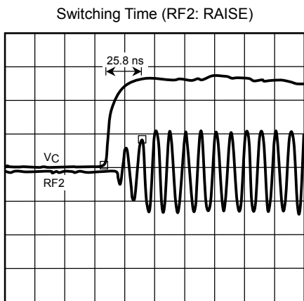
Time (20 ns/div)
