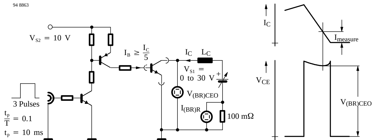
Figure 1. Test circuit for V_{(BR)CE0}
