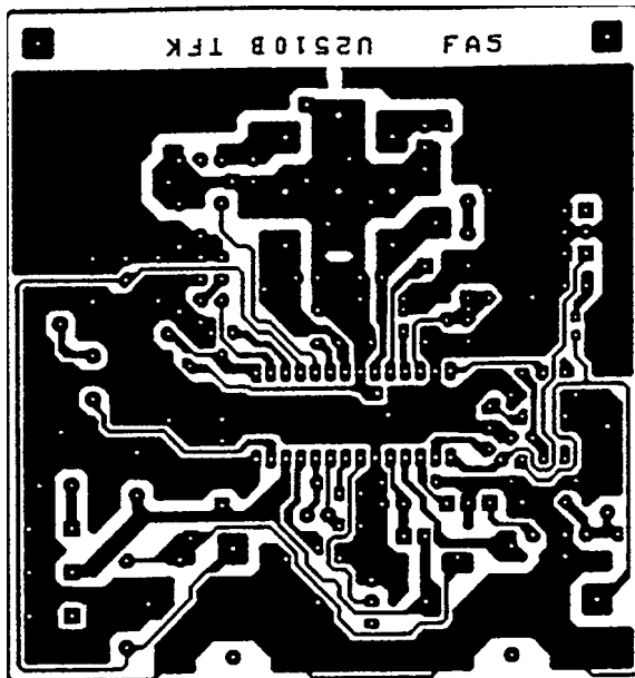
Figure 19. PC-board
