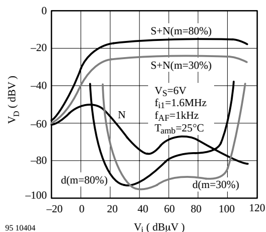
Figure 9. AM section: Demodulator output level
