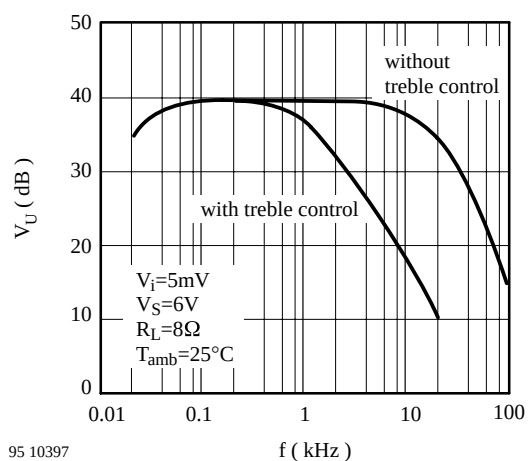
Figure 4. AF section
