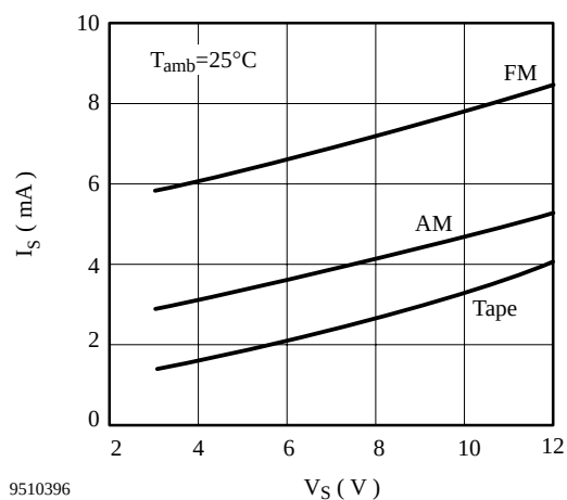
Figure 3. Quiescent current
