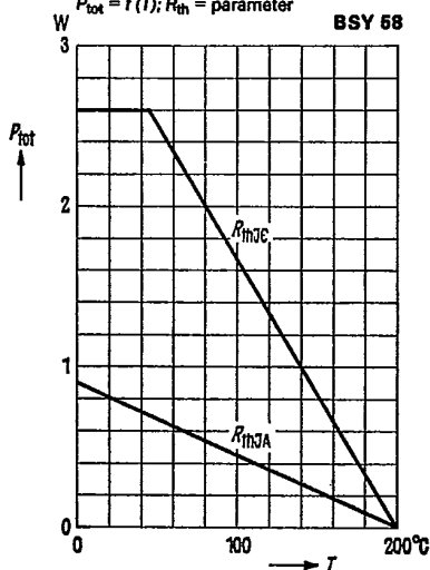
Total perm. power dissipation versus temperature P_{\text{tot}} = f(T); R_{\text{th}} = \text{parameter}
