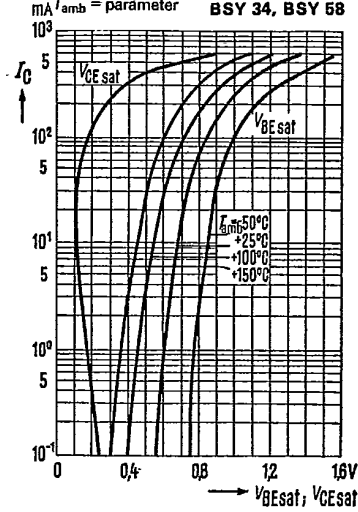
Saturation voltages V_{CEsat} = f(I_C); \eta_{FE} = 10 V_{BEsat} = f(I_C); \eta_{FE} = 10 T_{amb} = \text{parameter} BSY 34, BSY 58
