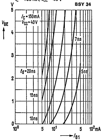
Delay time t_d I_C = 150 \text{ mA}; V_{CC} = 40 \text{ V}
